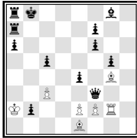
H#3 b)a7<->f7 (7+12)
